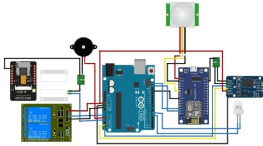
Gambar 2.3 Rangkaian Home Security
