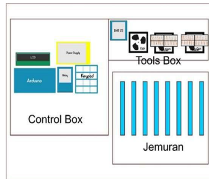
Gambar 7 Blok Diagram
