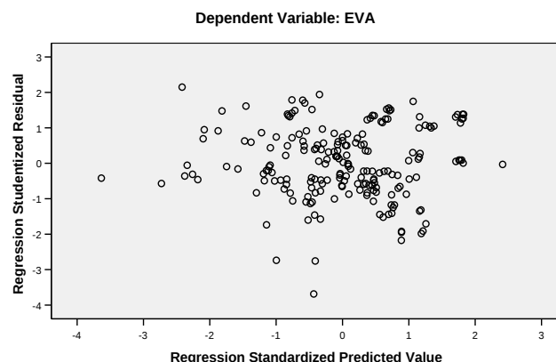
Gambar 4.1 Scatterplot
