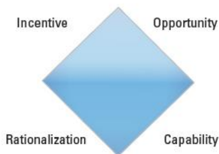
Gambar 2.1: Fraud Diamond
