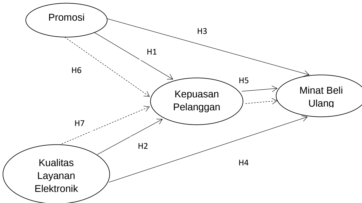
Gambar: Model Struktural
